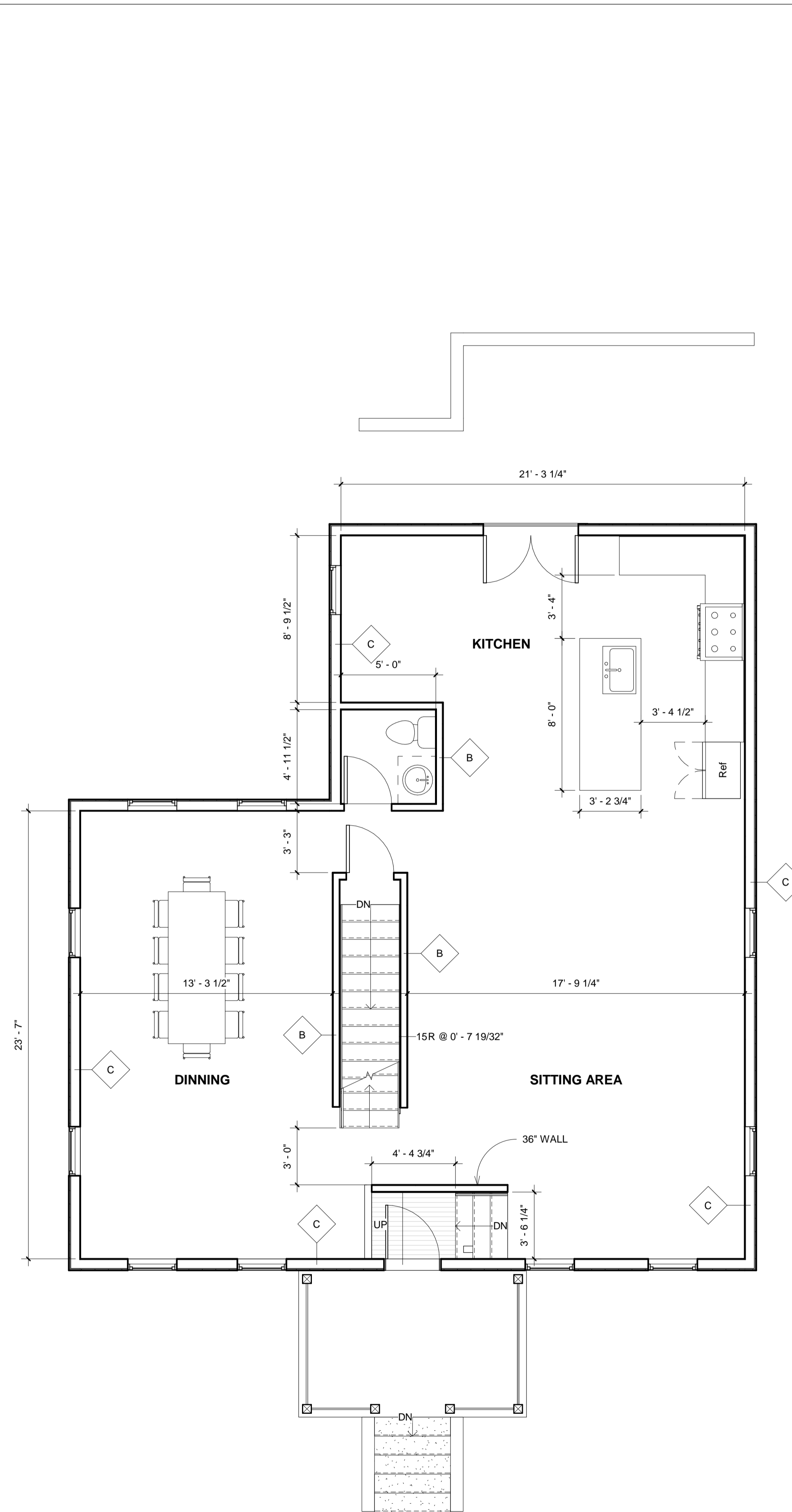
2 PROPOSED FIRST FLOOR PLAN 1/4" = 1'-0"
