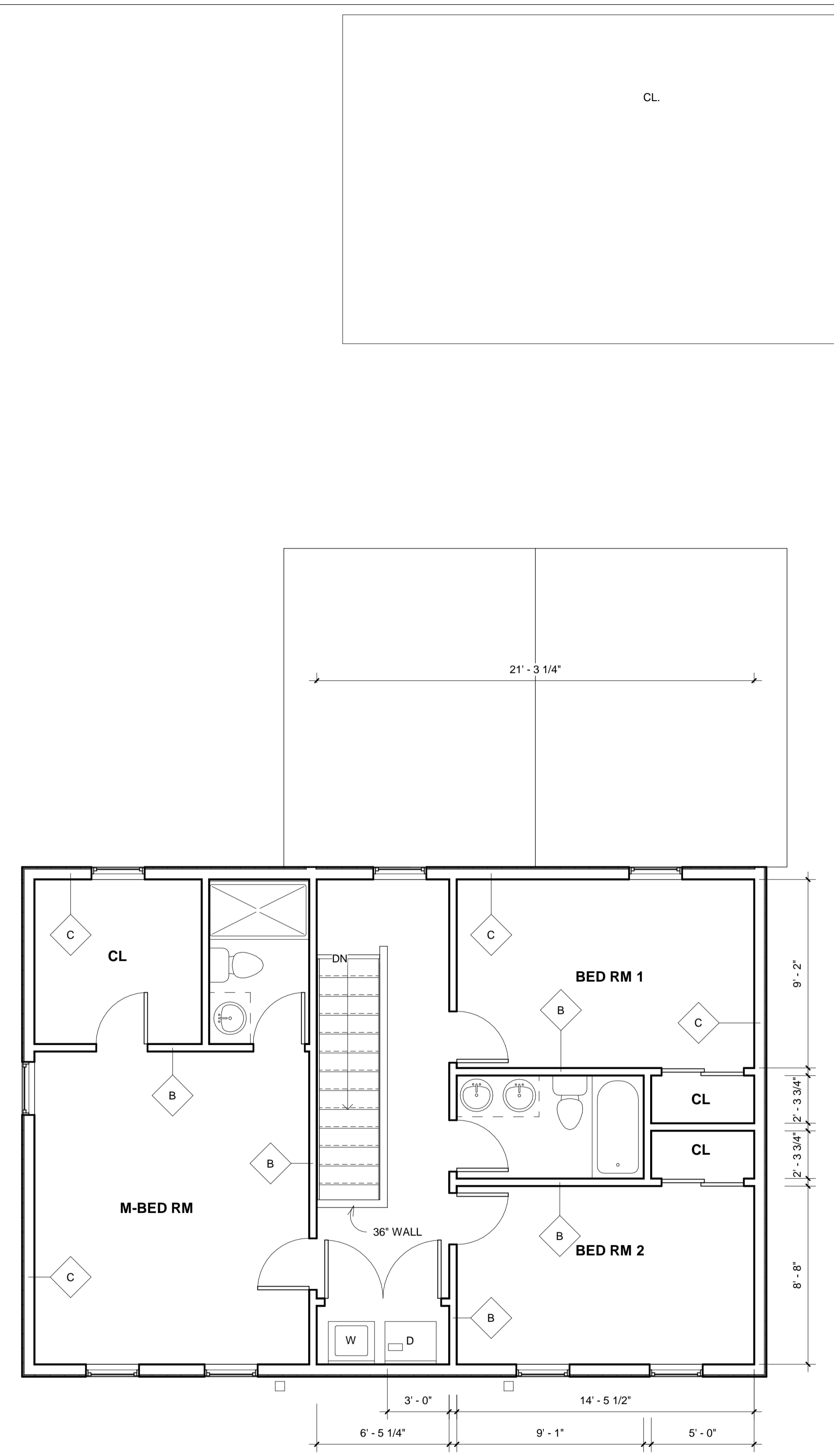
3 PROPOSED SECOND FLOOR PLAN 1/4" = 1'-0"
