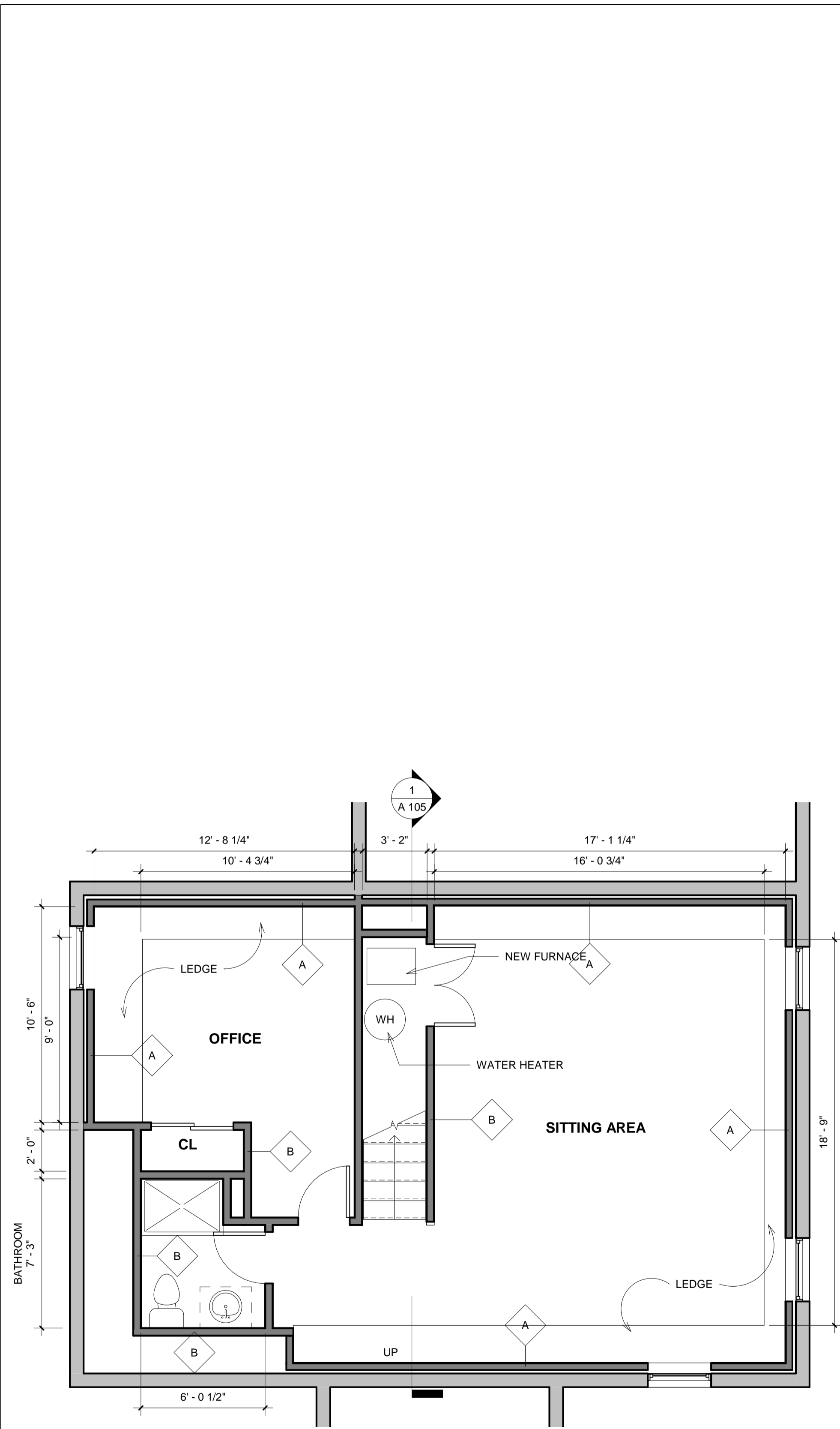
1 PROPOSED BASEMENT PLAN 1/4" = 1'-0"
